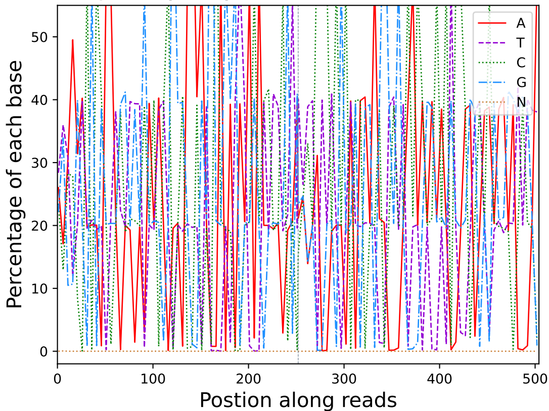
Base percentage along reads (R10727)
